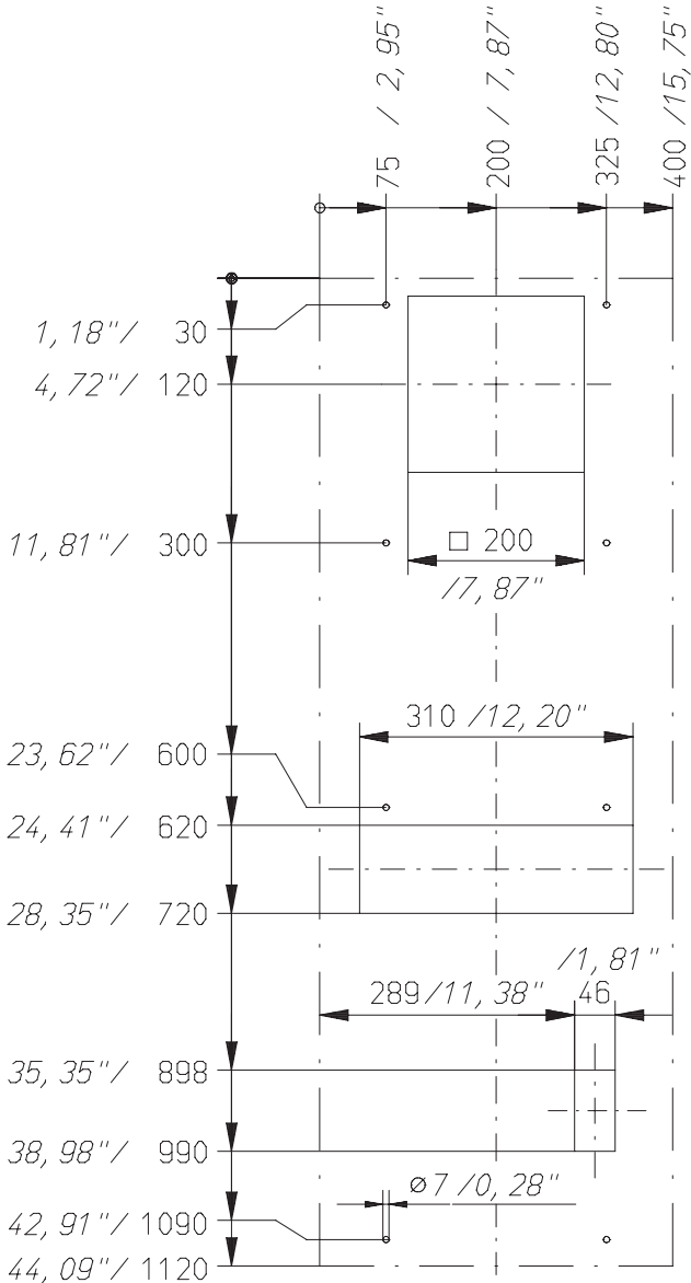
Drilling template external mounting
